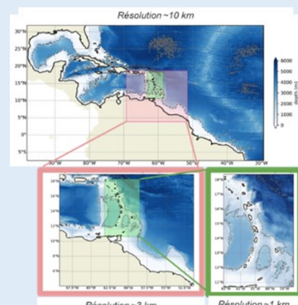
Fig. 3. NEMO configurations (nested grids) developed for the modeling of current and future climate and ocean circulation.
