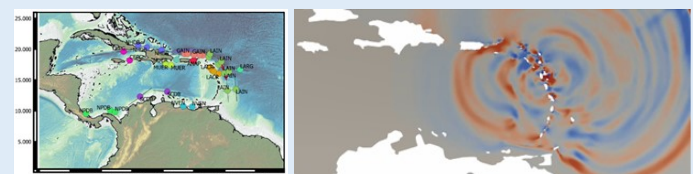
Fig. 6. Map of scenarios of tsunami sources (left). Example of a simulation of tsunami generation and propagation. Source inspired by Feuillet et al. 2011.
