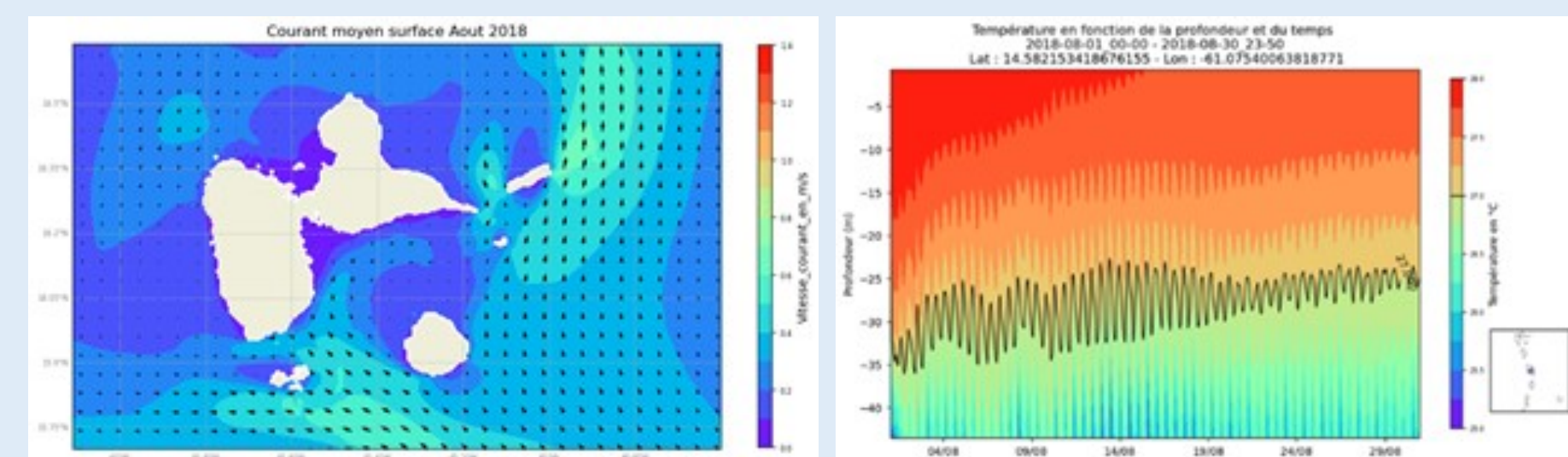
Fig. 4. Circulation modeling outputs: Mean surface current in August 2018 around Guadeloupe (left); variation of temperature with depth and time, evidencing internal waves (right).
