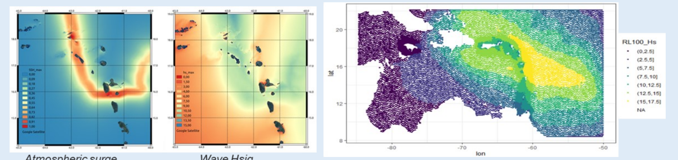
Fig. 5. Example of cat 5 hurricane simulation (Left) and 100y return period significant wave high (Hs, right).
